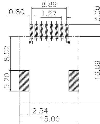
RECOMMENDED P.C.B LAYOUT TOP VIEW (COMPONENT SIDE)
