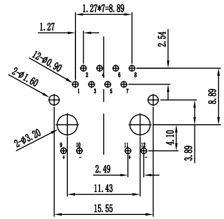
RECOMMENDED P.C.B LAYOUT TOP VIEW (COMPONENT SIDE)
