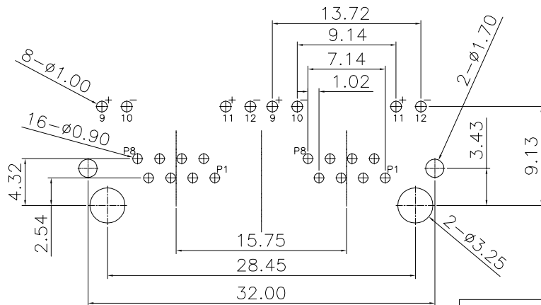
RECOMMENDED P.C.B LAYOUT TOP VIEW (COMPONENT SIDE)
